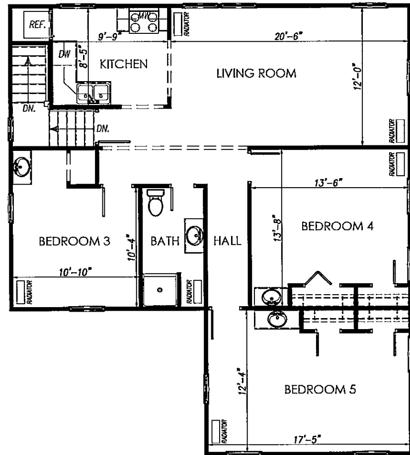
SECOND FLOOR
